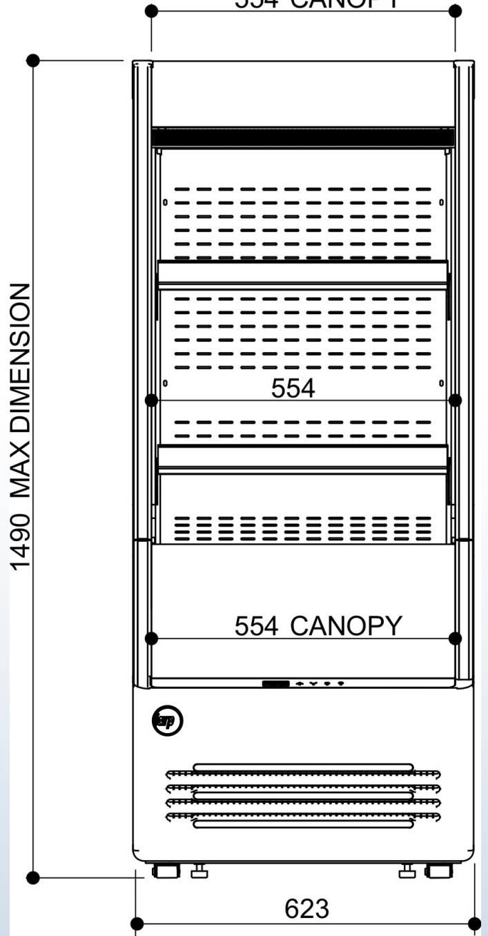
Frontal view 554 CANOPY
